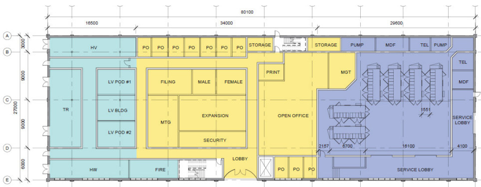
Scheme 2: Multi-Purpose Bldg Ground Level
